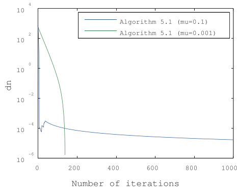
FIGURE 5. Behavior of d_n for Algorithm 5.1 when \mu = 10^{-1}, 10^{-3}
