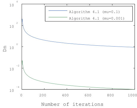
FIGURE 1. Behavior of D_n for Algorithm 4.1 when \mu = 10^{-1}, 10^{-3}
